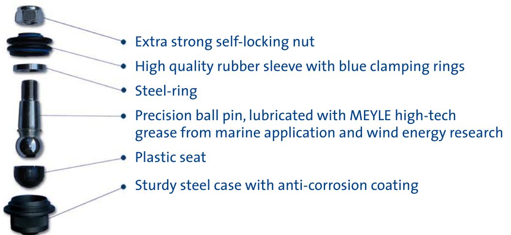
Exploded drawing ball joint
