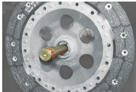
Image 6: 400 0111 10 in use
