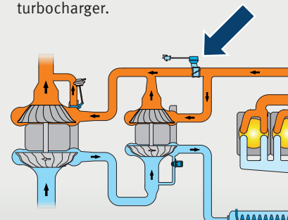
Register turbocharging (schematic)
