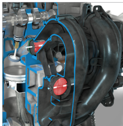
Flaps on the intake manifold
